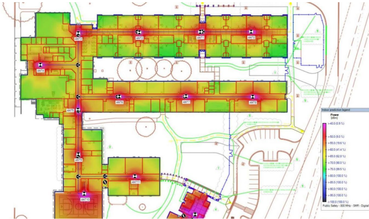
Sample Heatmap for Installed BDA System in a Building with Drywall
